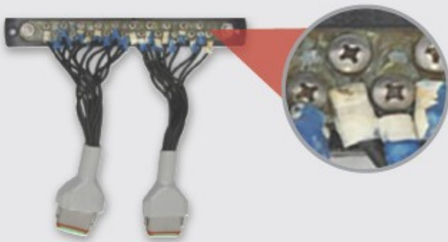
Standard bus bar with corrosion
